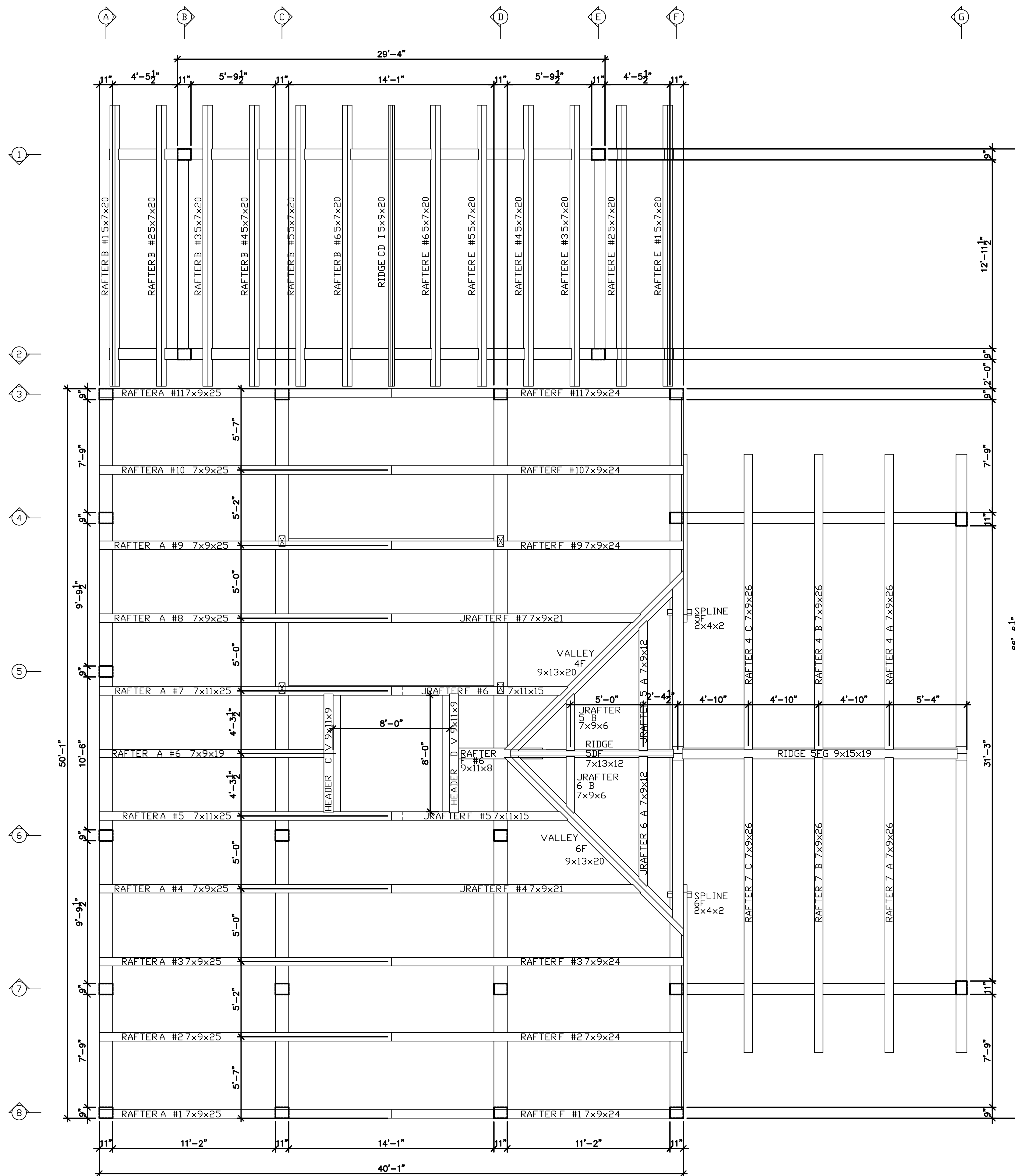
POST & RAFTER PLAN
